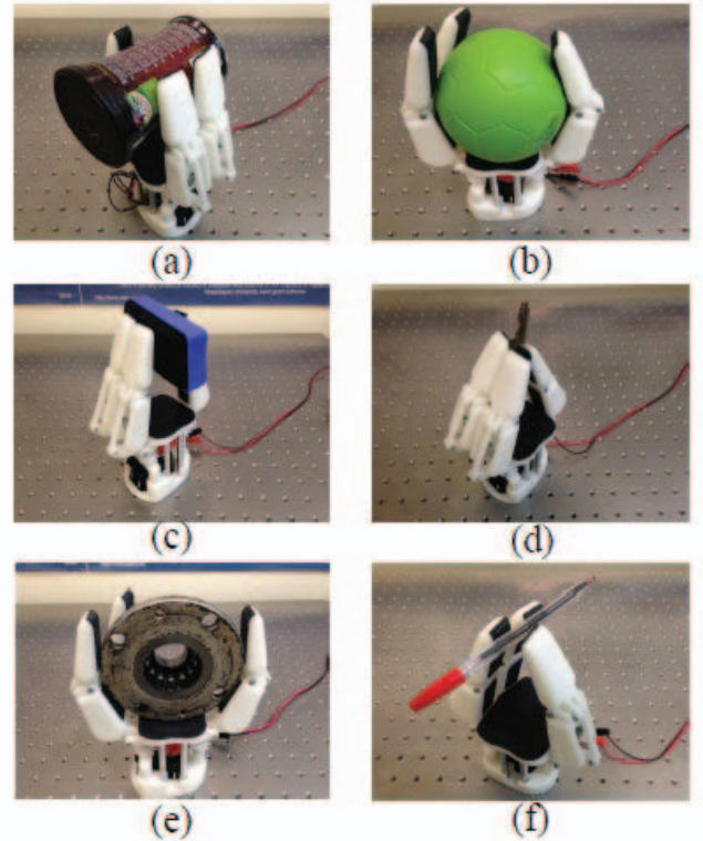
Fig. 8. Grasping of different objects of the robotic gripper prototype: (a) Cylindrical grasp. (b) Spherical grasp. (c) Planar grasp. (d) Fingertip grasp. (e) High payload, large shape grasp. (f) Low payload, small shape grasp.
